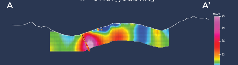
IP Chargeability
